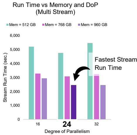
Figure 3: Multi-stream DoP
